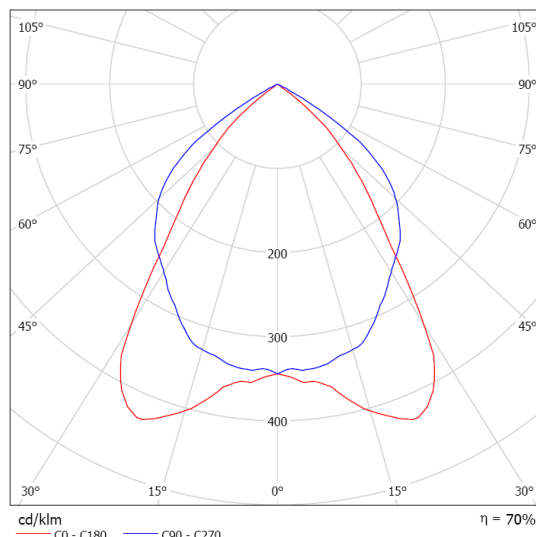
1X35W
